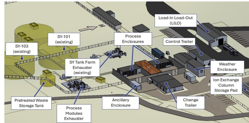
Conceptual design: West Area Risk Management Project
