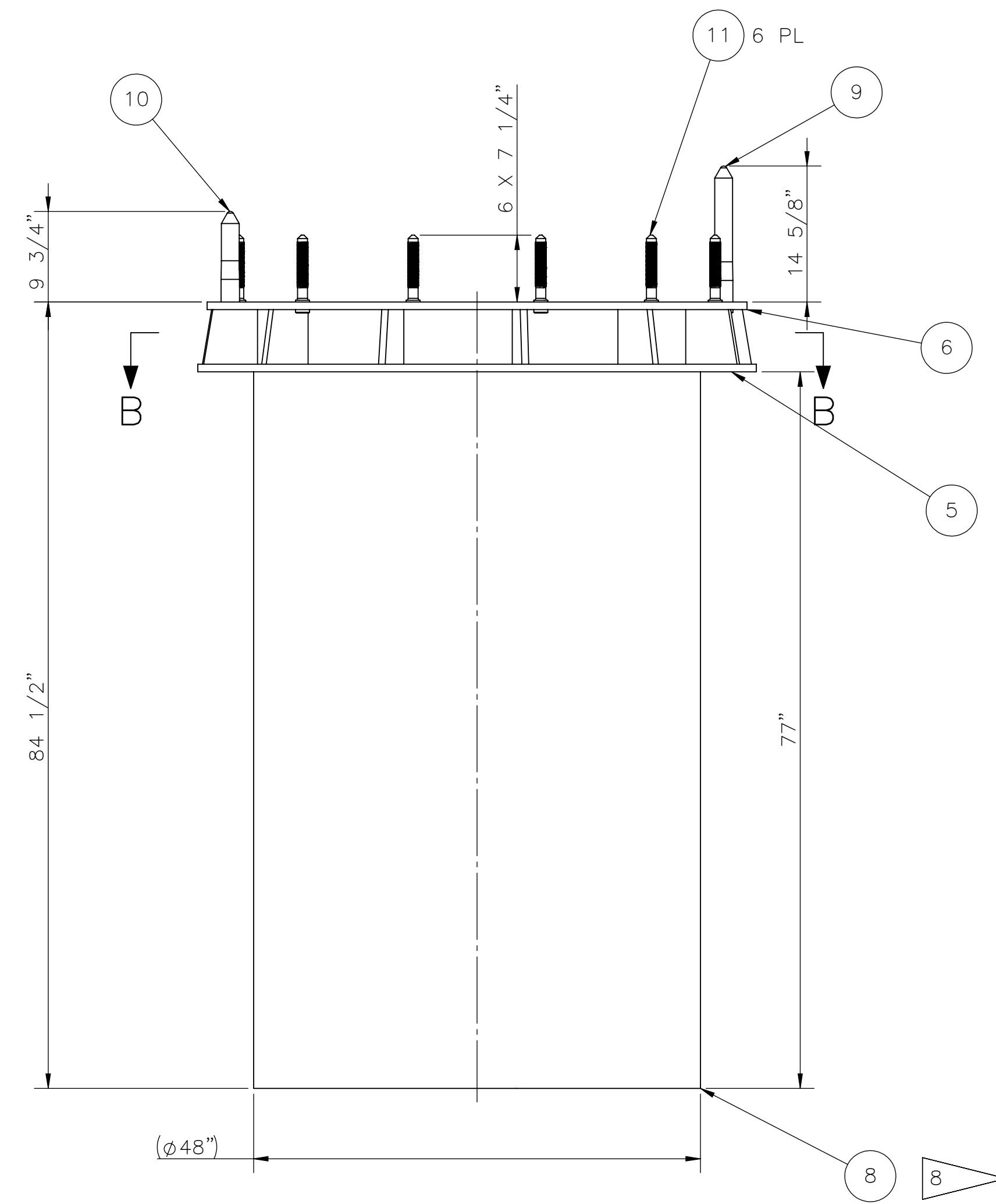
1 PWST 48 INCH RISER ASSEMBLY SCALE: 1"=1'-0" PART DETAILS ON SHT 3
